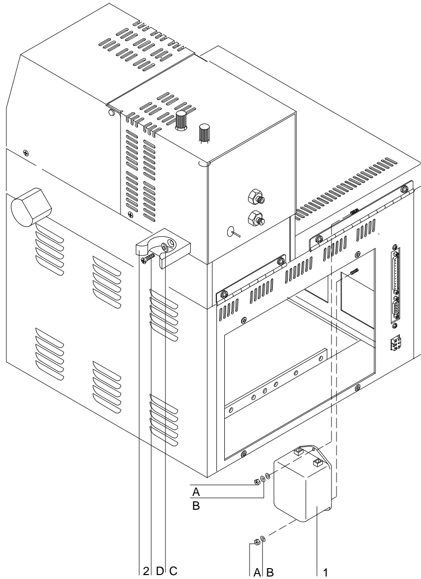
Figure 1-2. Removing the Power Supply Filter
