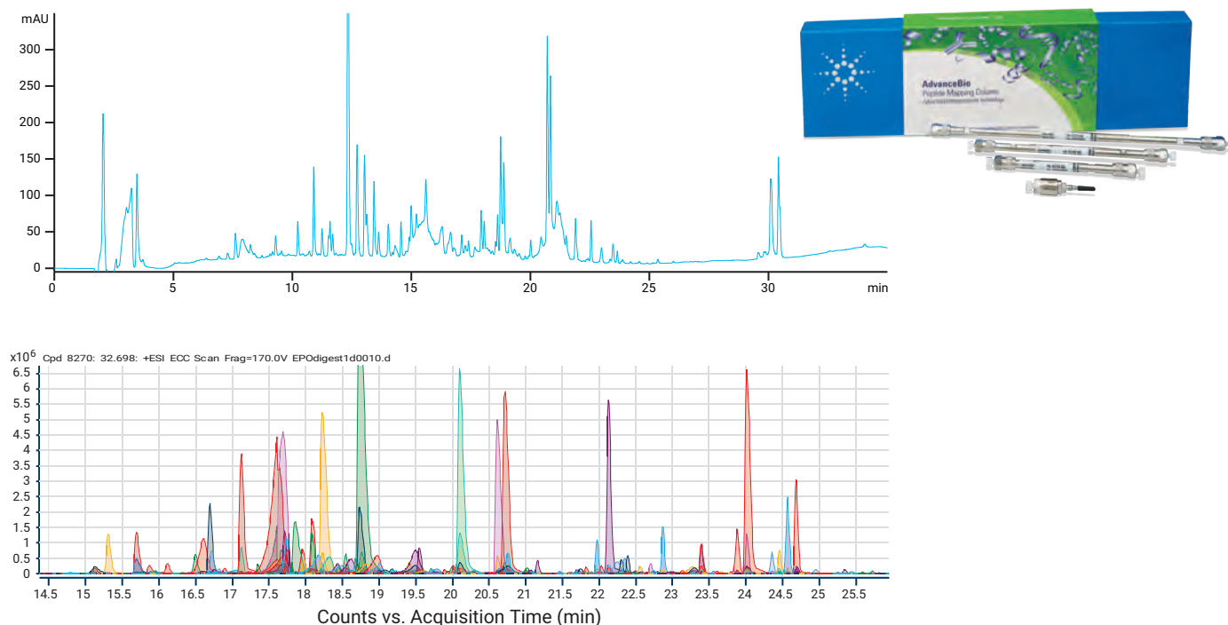
Figure 12. The top chromatogram displays a fully optimized EPO digest peptide mapping separation performed on a 2.1 x 150 mm AdvanceBio Peptide Mapping column. The bottom chromatogram shows the qualitative analysis (using a molecular feature extractor) for sequence coverage generated by an Agilent Q-TOF.
