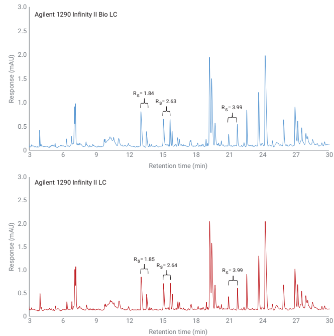
Figure 1. Chromatograms of a tryptic digest of the NISTmAb separated by the Agilent 1290 Infinity II Bio LC and the Agilent 1290 Infinity II LC with the same method (Table 1).
